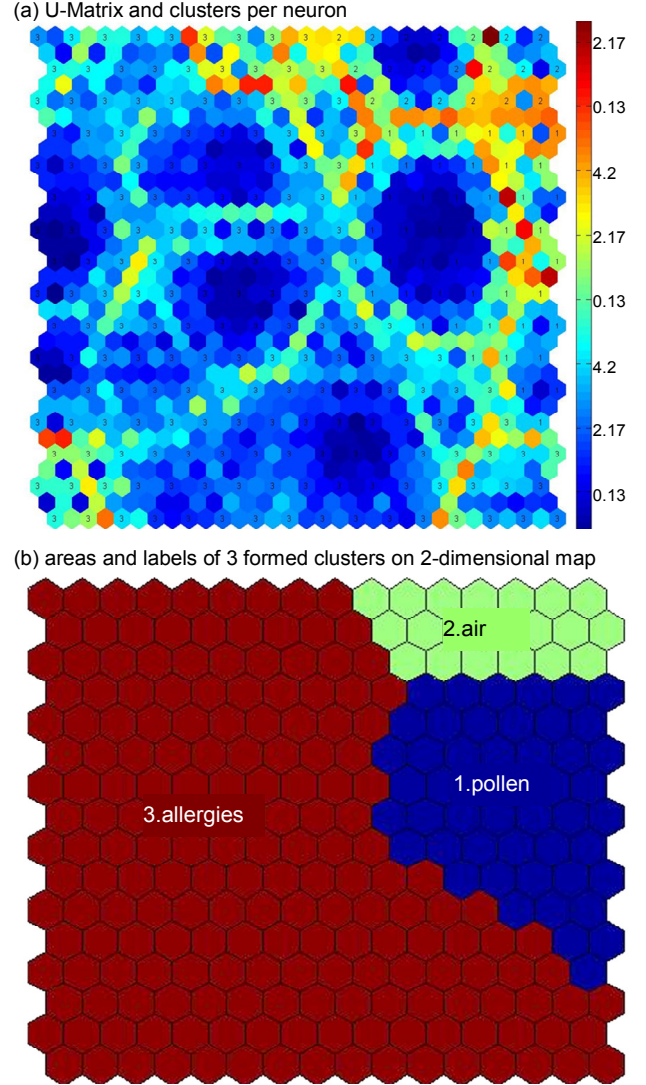
Figure 7. (a) U-Matrix and clusters per neuron, (b) areas and labels of 3 formed clusters on 2-dimensional map.
