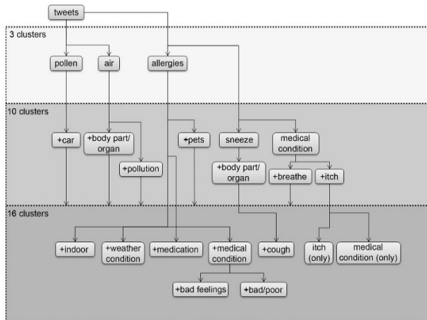
Figure 13. The hierarchy of concepts derived after three levels of clustering.
